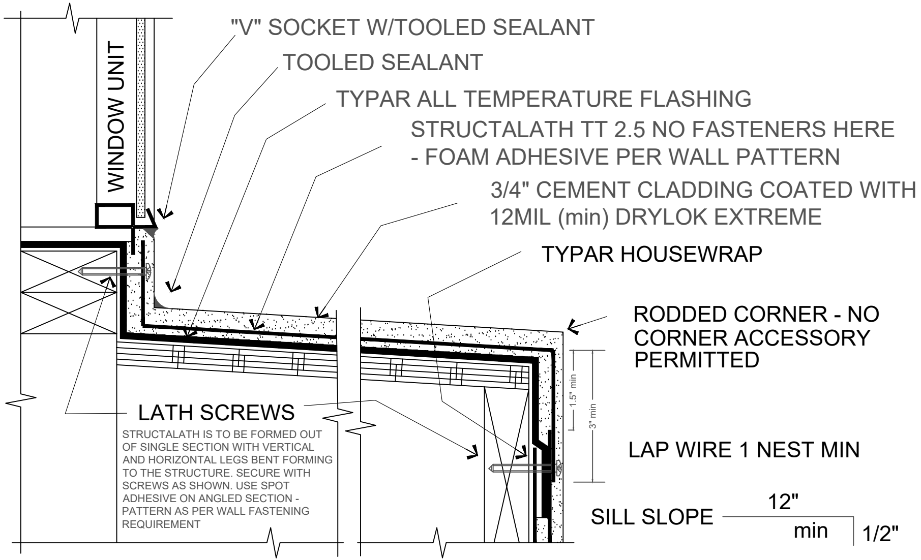
SCS 07-04 SELF-ADHERED FLASHING LEDGE, POTSHelf OR SHOULDER
