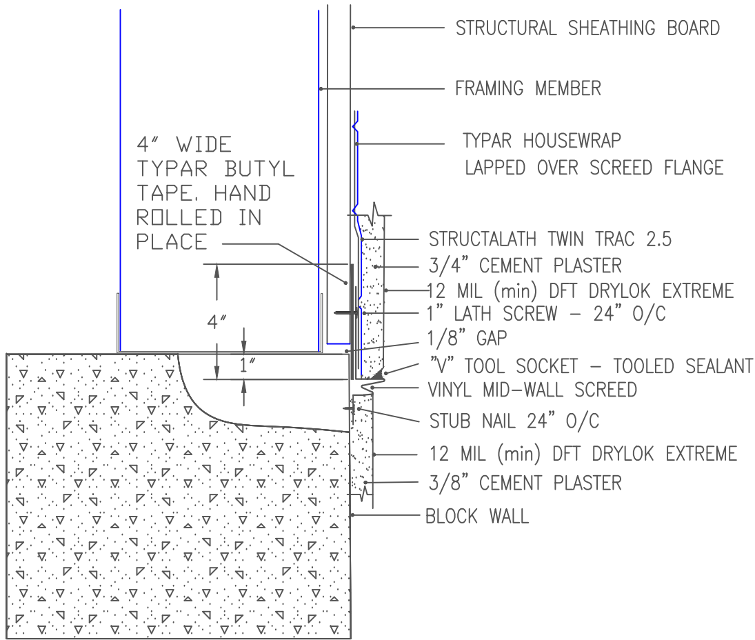
SCS 04_02 MIDWALL FRAME TO CMU USING A TRANSITION SCREED
